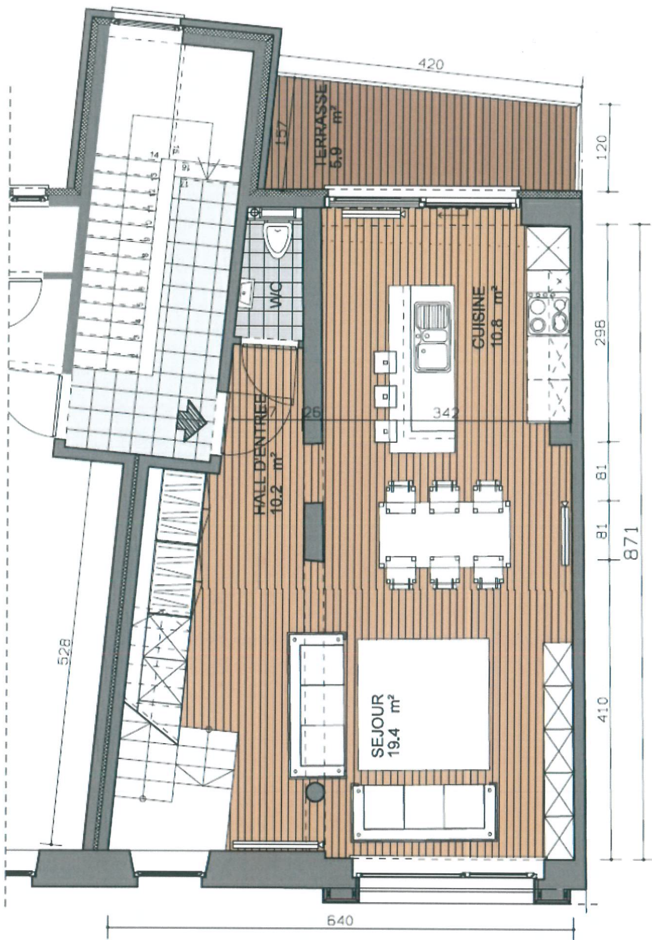
PLAN NIVEAU +1
